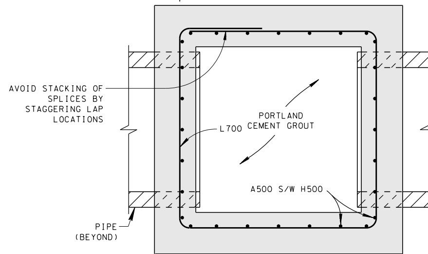
SECTION E-E
